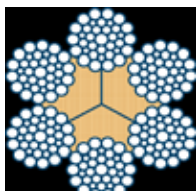
6 Round Strands
