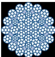
16 Round Strands
