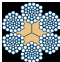
6 Triangular Strands
